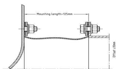
Design B Flexible connection with loose flange
