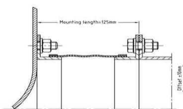
Design A Flexible connection with angle frame
